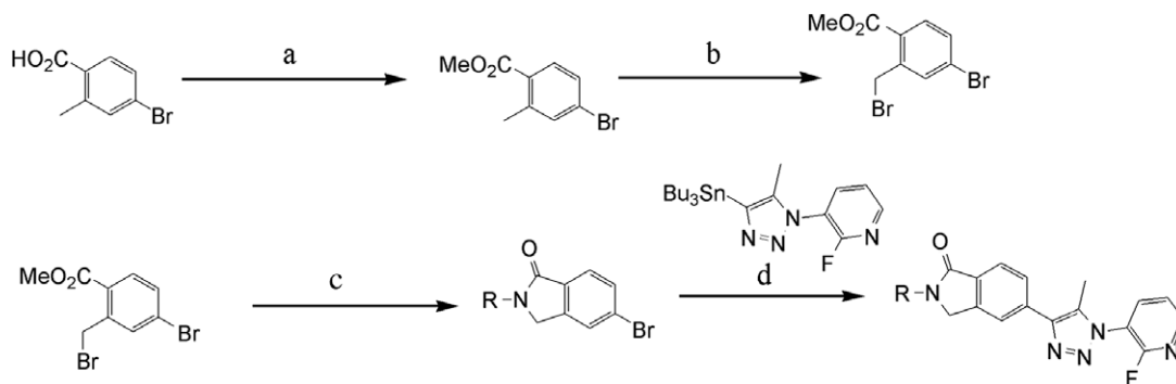
Scheme 2. Preparation of isoindolinone derivatives. Reagents and conditions: (a) concd \text{H}_2\text{SO}_4 , MeOH, reflux; (b) N -bromosuccinimide, benzoylperoxide, \text{CCl}_4 , reflux; (c) \text{R-NH}_2 , TEA, toluene, reflux; (d) \text{Pd}(\text{PPh}_3)_4 , DMF, 115^\circ\text{C} .
